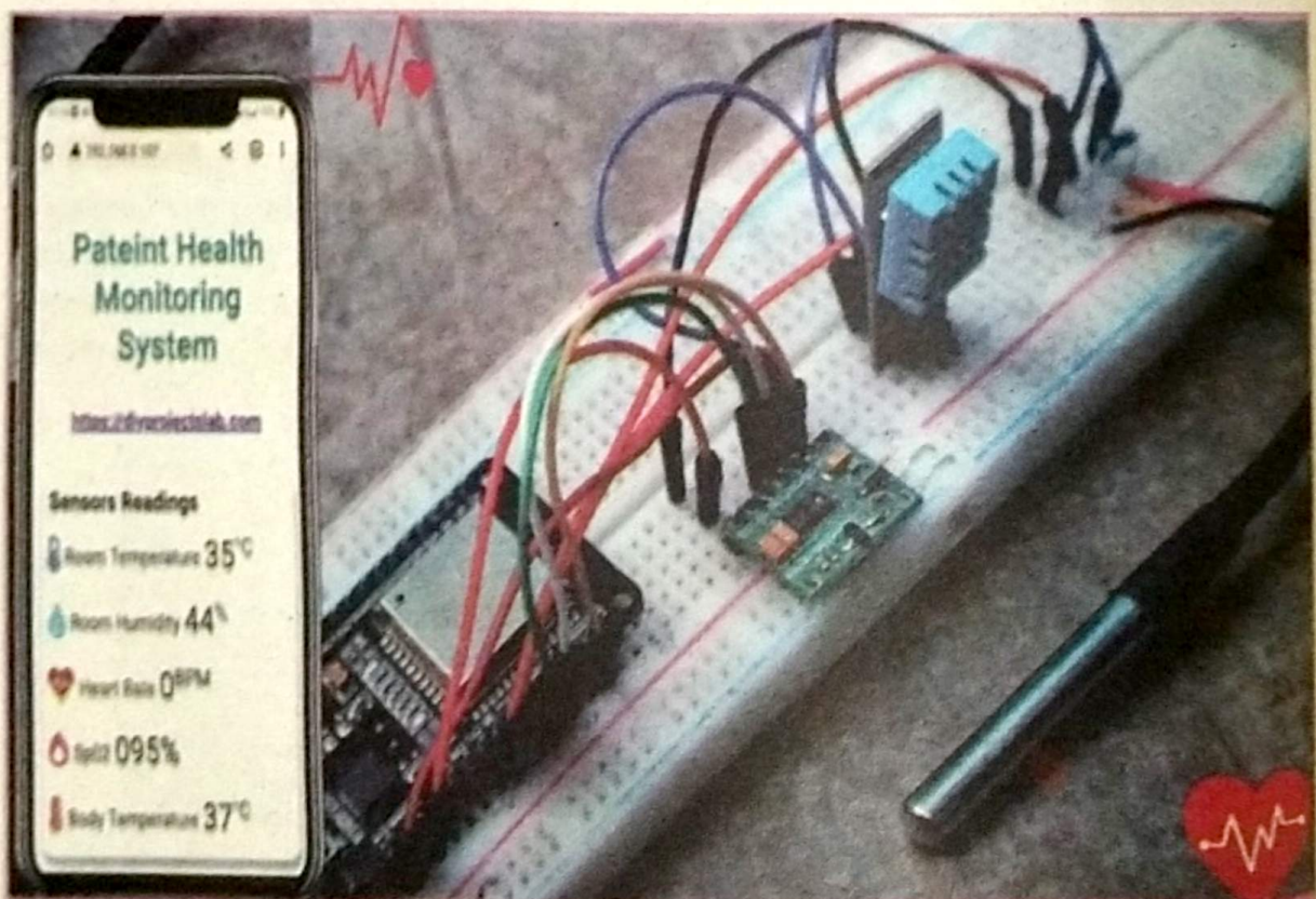
Fig.5.7: IoT based Patient Health Monitoring System
