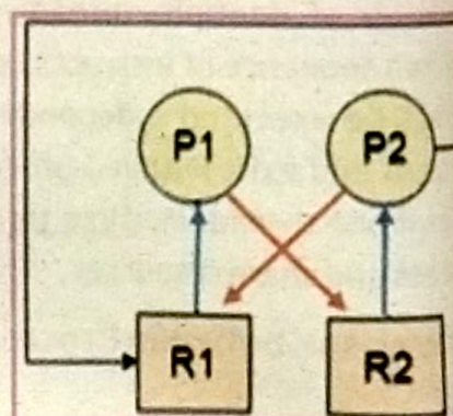
Fig.1.23: Deadlock
