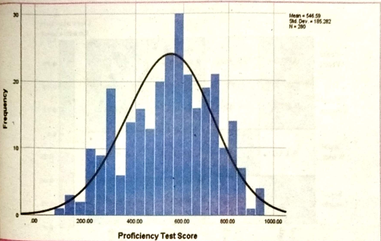
Fig.4.18: Histogram
