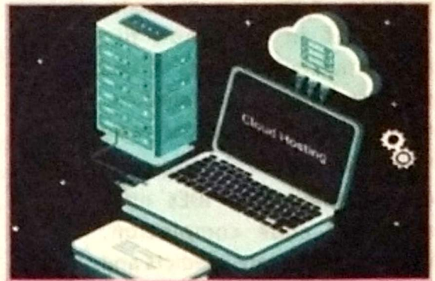
Fig. 1.28: Cloud Hosting
