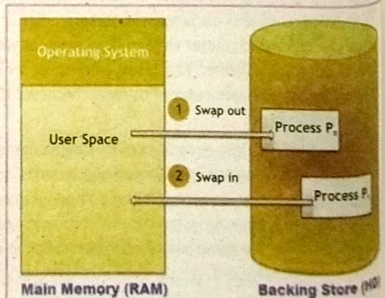
Fig.1.5: Memory Management
