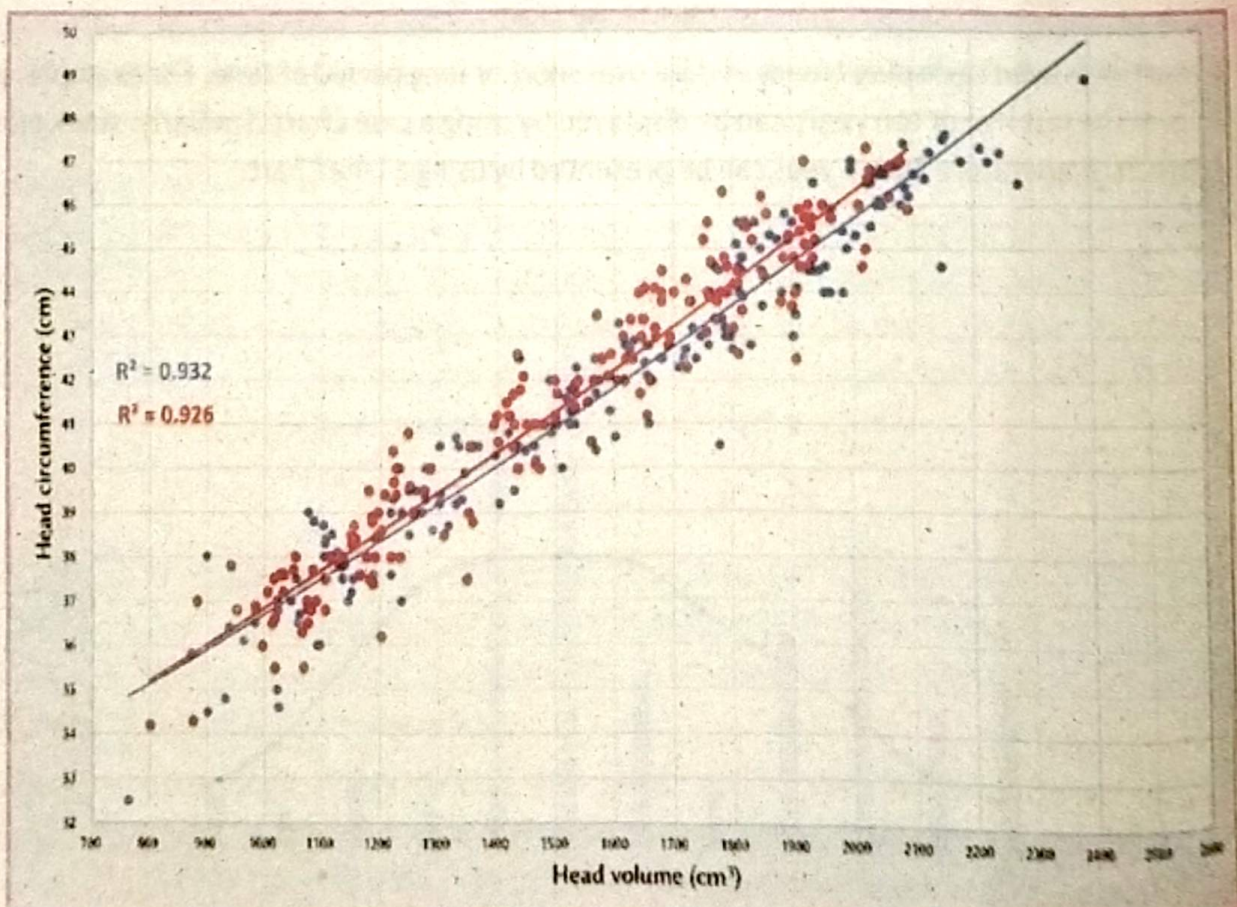
Fig.4.17: Scatter Plot
