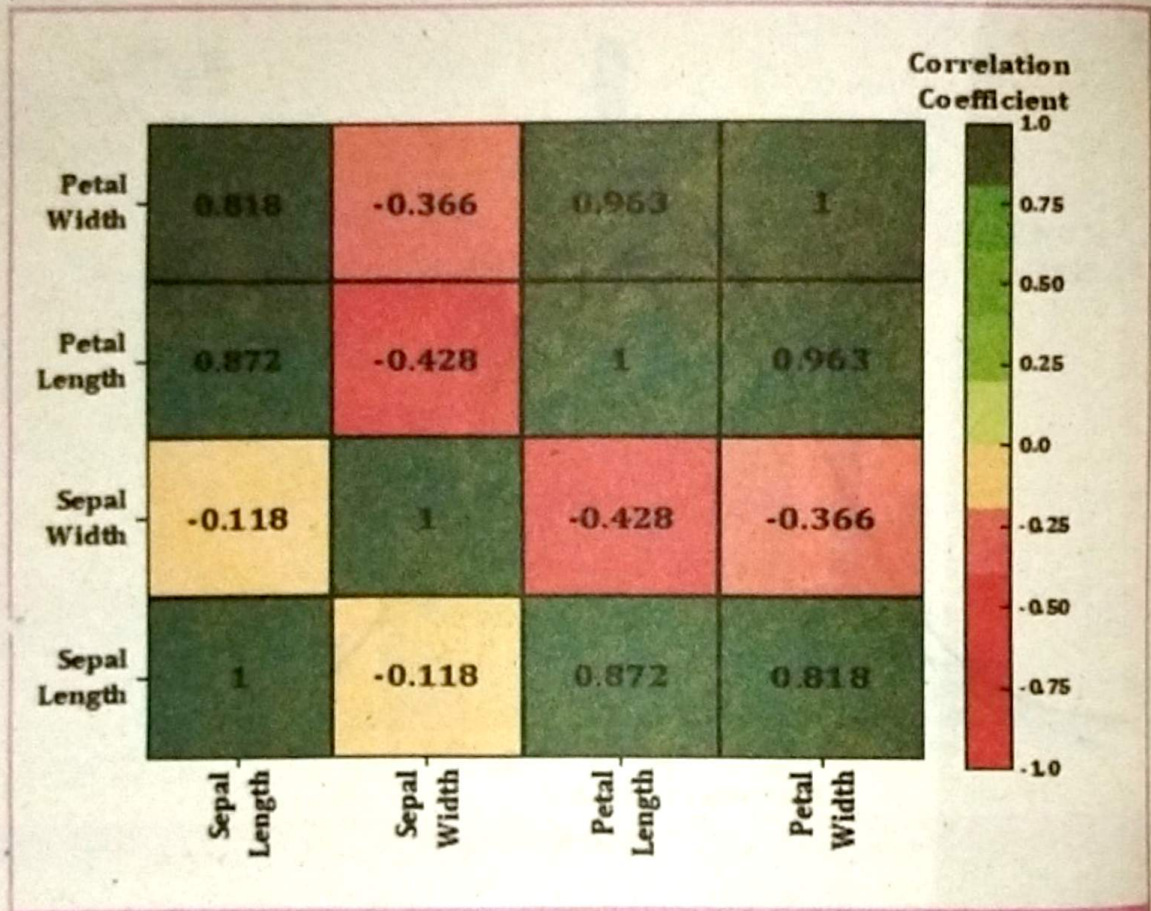
Fig.4.20: Heatmap
