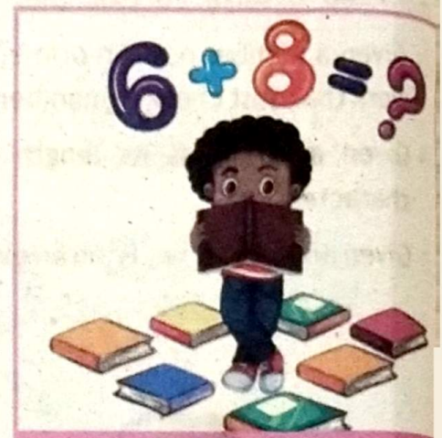
Fig.2.7: Addition
