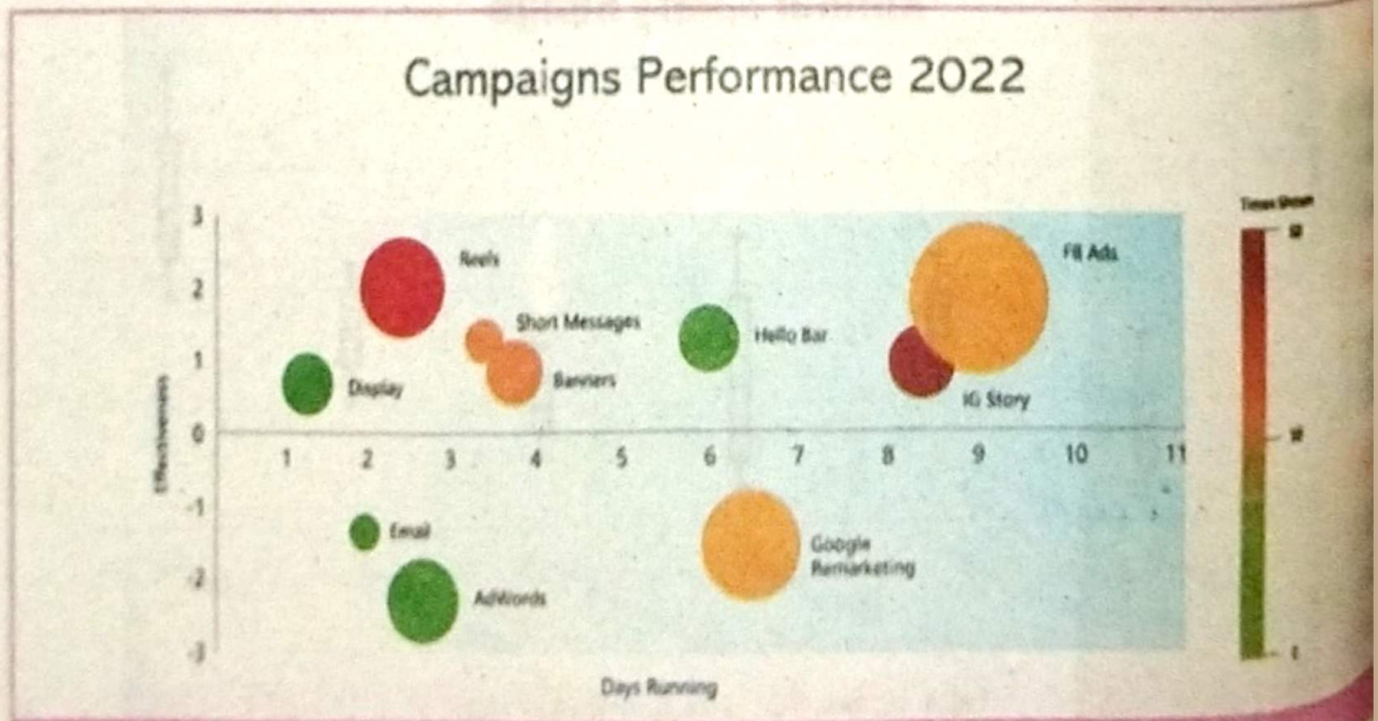
Fig.4.21: Bubble Chart
