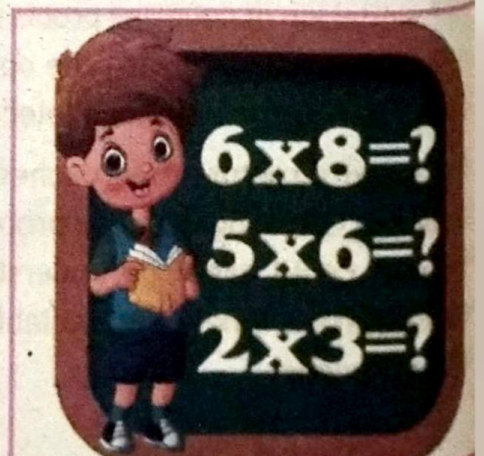
Fig.2.8: Multiplication
