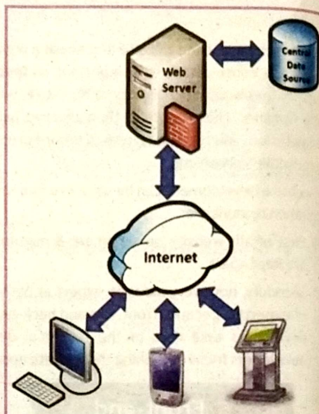
Fig.2: Client-Server architecture
