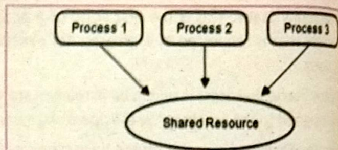
Fig.1.22: Process Synchronization
