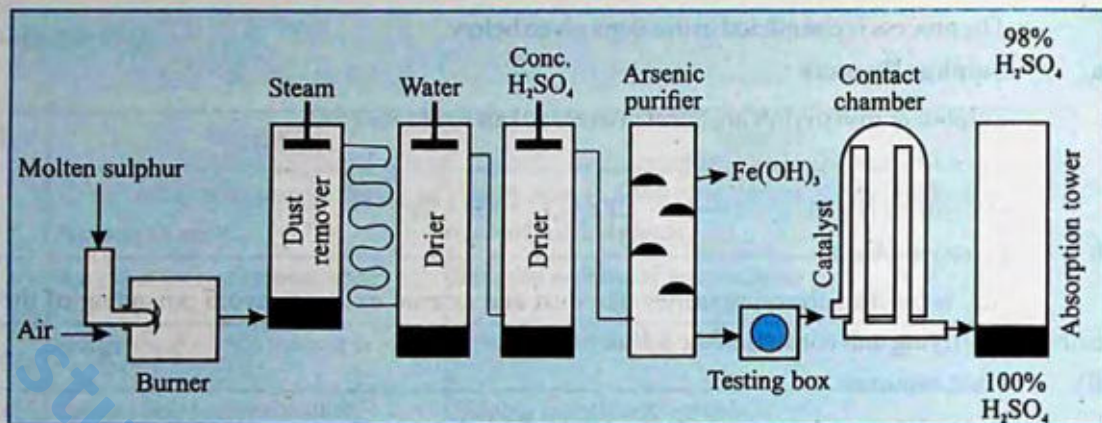
Fig.4.5 Contact Process
