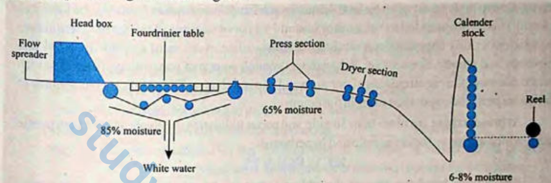
Fig. 15.4 Fourdrinier paper making machine
