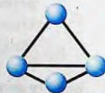
Fig.4.3 White phosphorus
