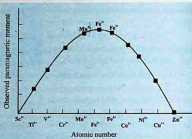
Fig 6.4 Variation in the paramagnetic effect shown by the selected ions across the first transition series
