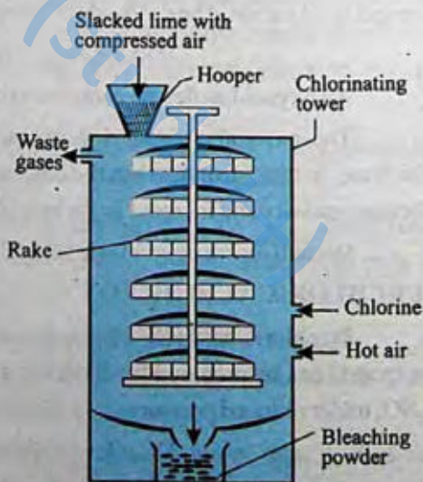
Fig. 5.3 Beckmann's Method
