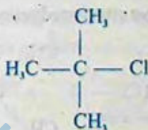
2-Chloro-2-methylpropane
