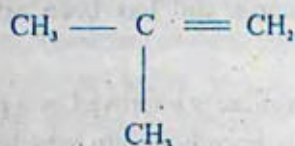
2-Methylpropene (Isobutylene)
