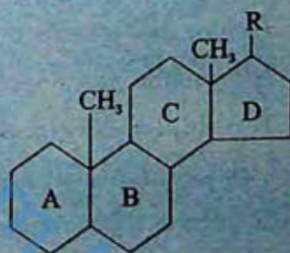
Structure of Steroid Nucleus
