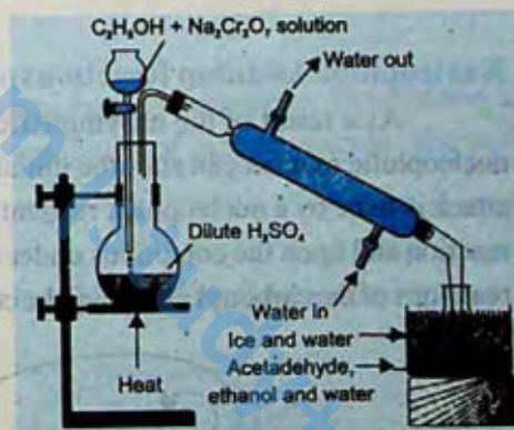
Fig. 12.2 Preparation of Acetaldehyde
