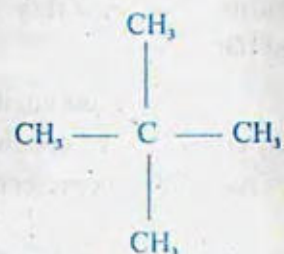
2, 2, 4-Dimethylpropane (neopentane)
