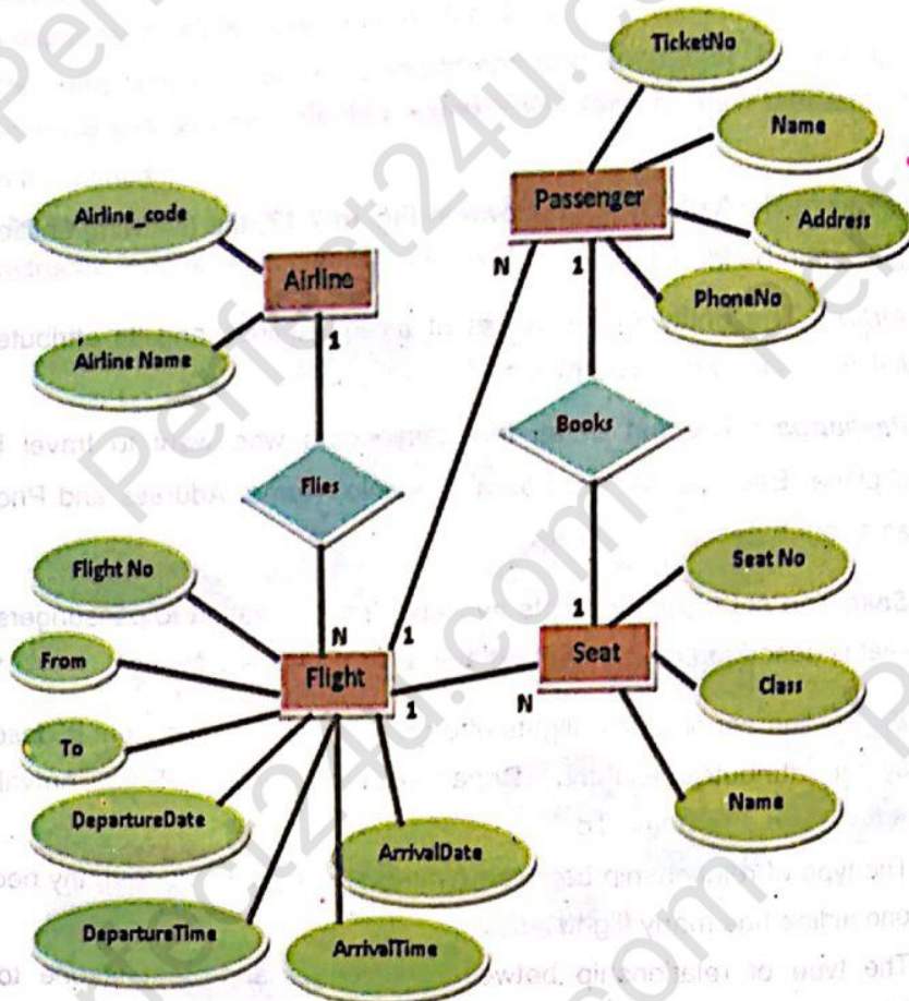
Figure 7.20 E-R Diagram for Ticket Booking System
