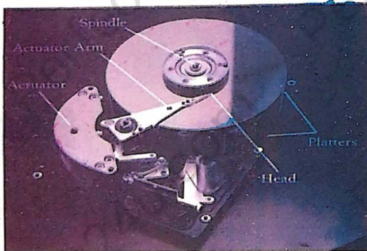
Figure 2.10 Working of Hard disk drive (HDD)
