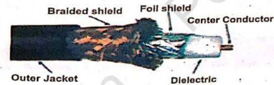
Figure 5.9 Coaxial Cable
