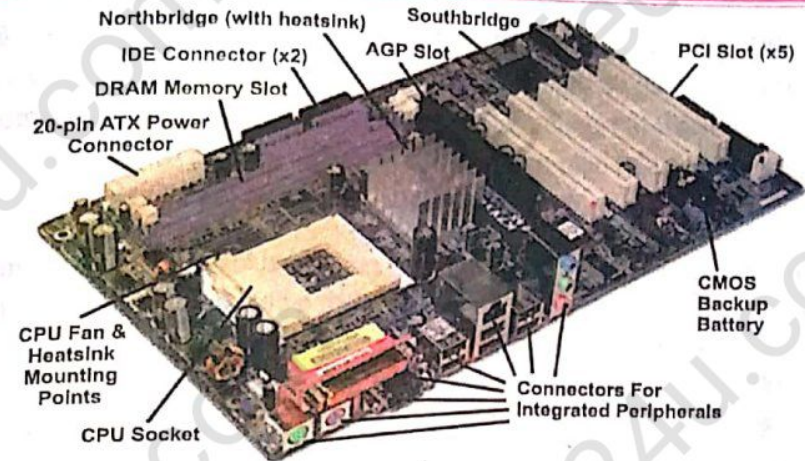
Figure 4.5 A Motherboard
