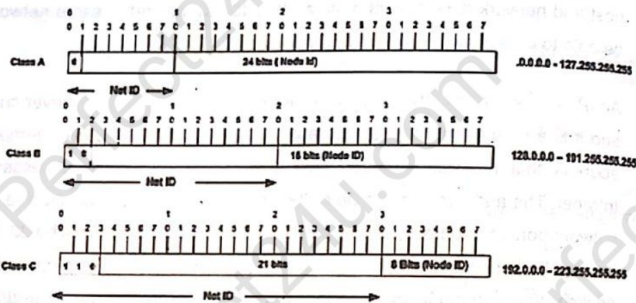
Figure 5.30 Classes of IP Addresses
