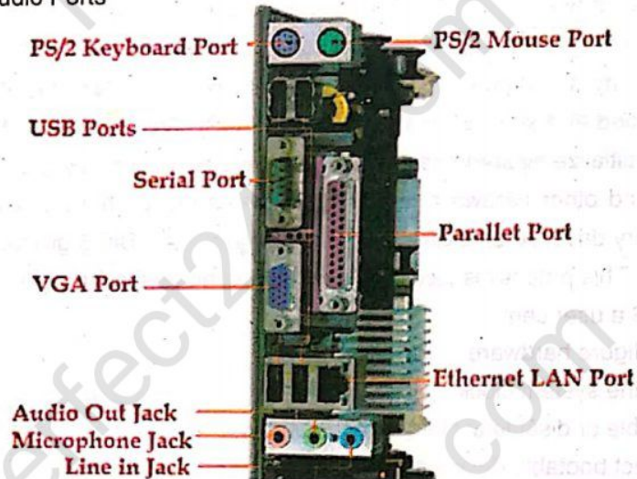
Figure 4.6 Ports
