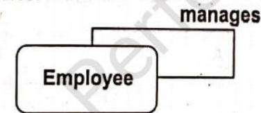
Figure 7.7 Unary/Recursive relationship
