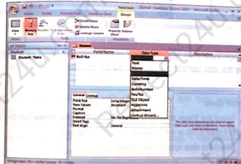
Figure 8.8 Fields in Design View
